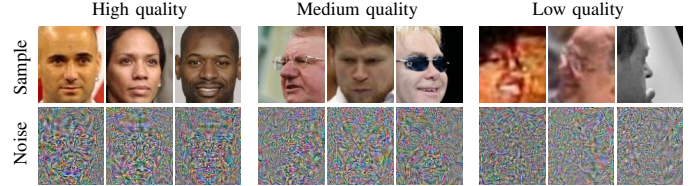
Fig. 1. Visualization of adversarial noise as a function of image quality. A clear difference can be observed in the characteristics of the adversarial noise between images of different quality. Higher quality images produce noise masks with a more distinct face-like pattern, while the lower quality masks are closer to random noise. FaceQAN takes advantage of the presented observations to estimate the quality of the input images.
